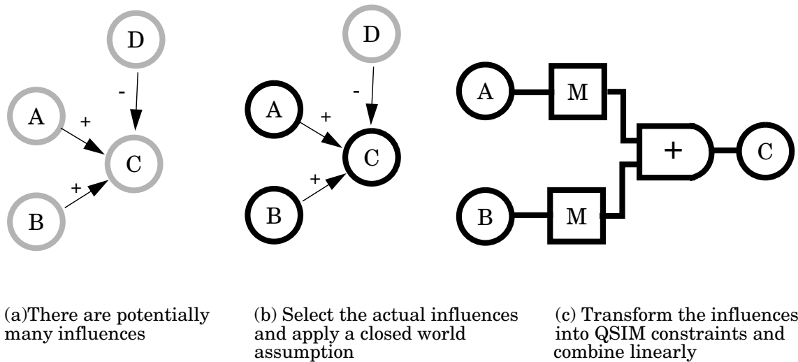
Figure 3. QPC transforms QPT influences into QSIM constraints
